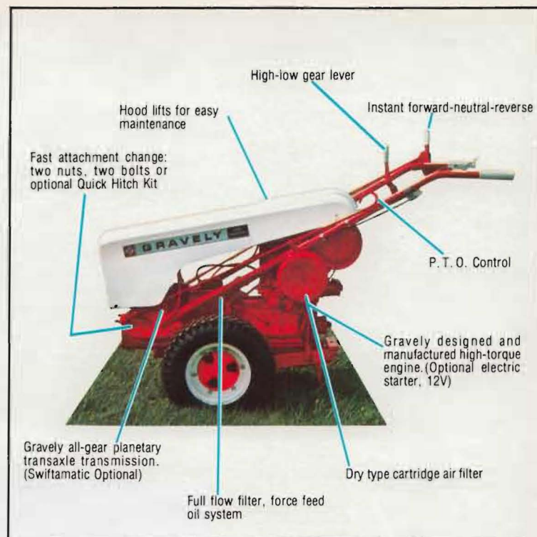
7.6 HP TRACTOR
