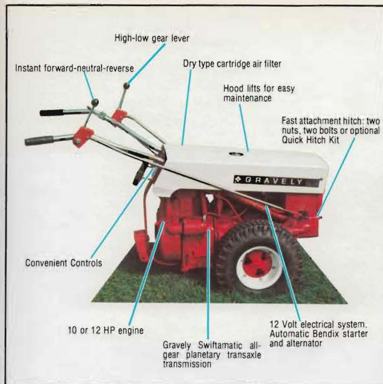
10 or 12 HP TRACTOR
